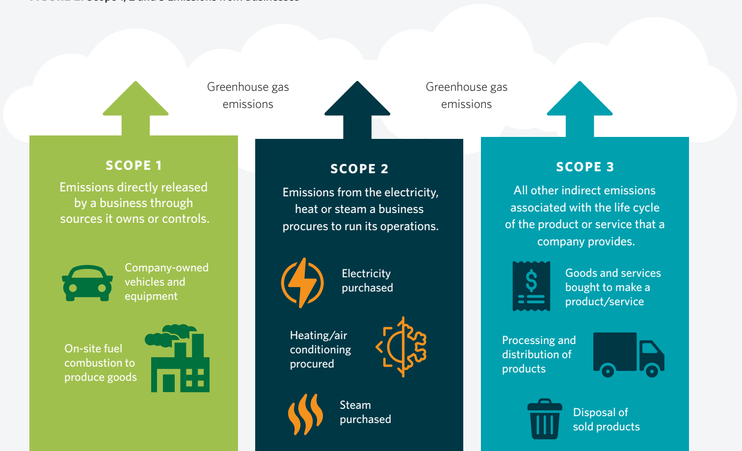
FIGURE 2: Scope 1, 2 and 3 Emissions from Businesses
