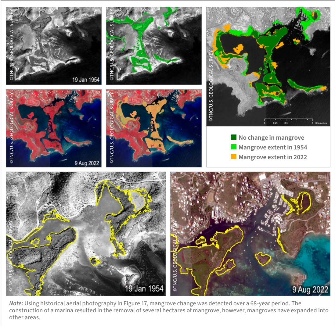
Figure 17. Historical aerial photography and mangrove change detection in Saint Thomas East End Reserve, the United States Virgin Islands
