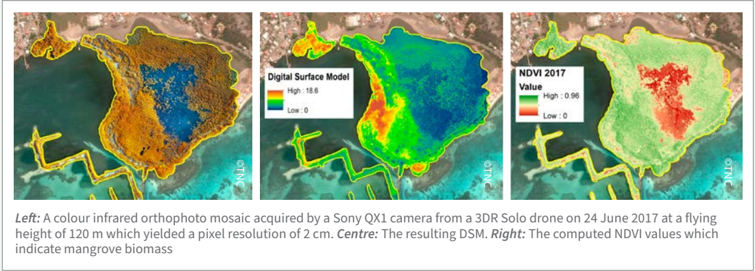
Figure A3.4 A colour infrared orthophoto mosaic, the resulting DSM and computed NDVI values of Ashton Lagoon, Saint Vincent and the Grenadines
