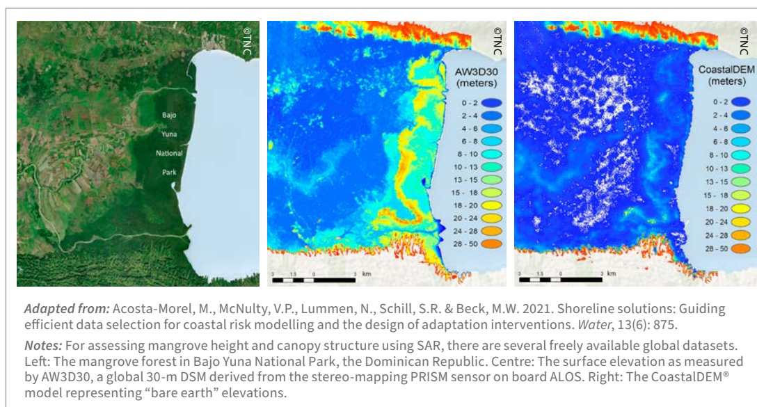
Figure 21. Comparison of global digital elevation models (AW3D30 and CoastalDEM®) for mangroves in Bajo Yuna National Park, Dominican Republic
