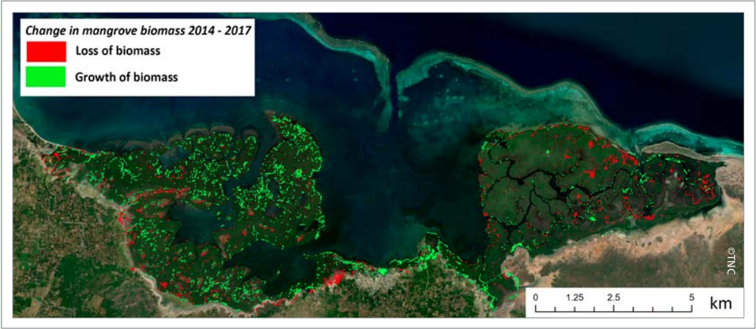
FIGURE A2.3 NDVI biomass change detection in Forte Liberté Bay and Lagon aux Bouefs from 2014 to 2017
