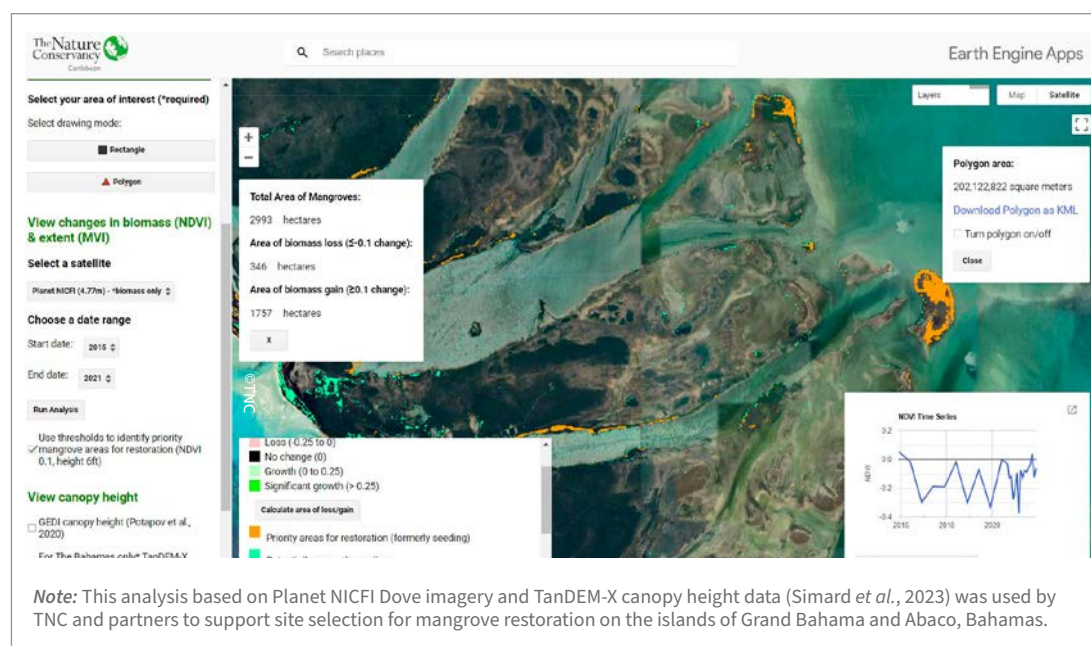
Figure 44. The Blue Carbon Explorer's example of mangrove restoration prioritization in eastern Grand Bahama, 2015–2021
