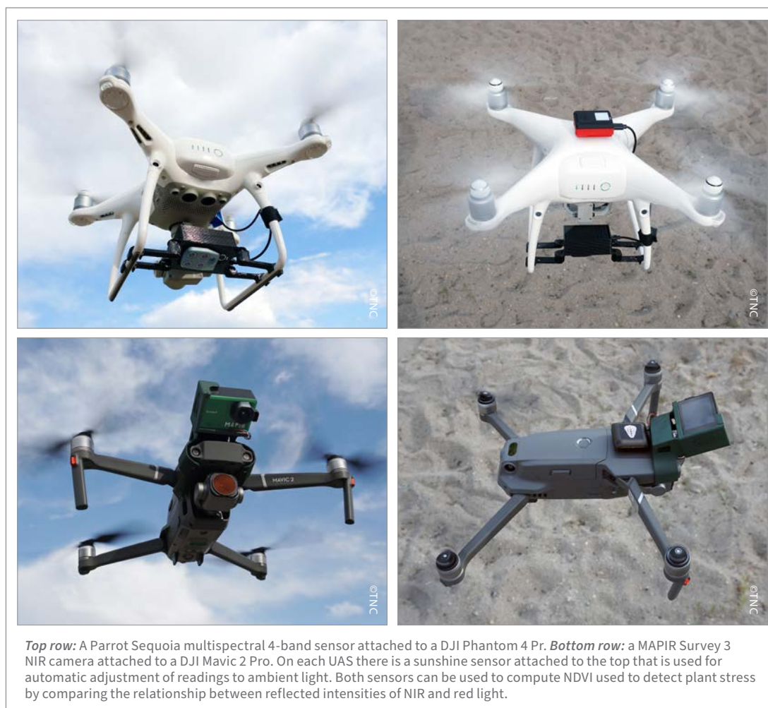
Figure 25. Two cost-effective UAS platforms with supplementary infrared sensors attached for assessing mangrove extent and health
