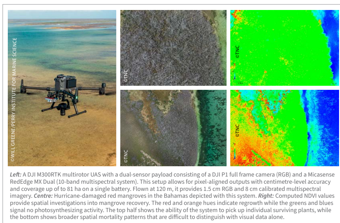
Figure 39. Using a DJI M300RTK multirotor UAS with a Micasense RedEdge MX to capture and compute NDVI to track mangrove recovery following a hurricane
